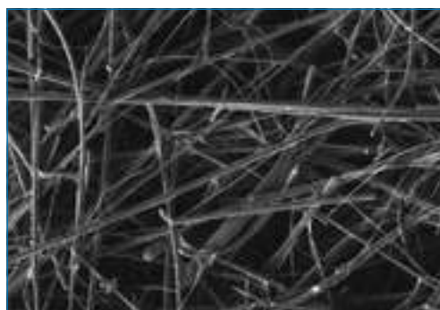
Natural Fiber Cellulose media, as seen under the scanning electron microscope.
